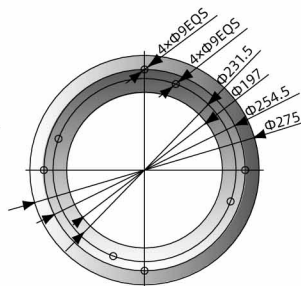
SHR-6U-ST~SHR-24U-ST
