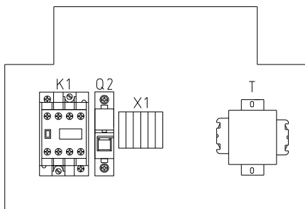
Control box elec. mount plate
